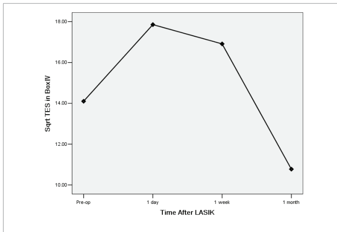
Figure 2: Changes in Sqrt TES in the box IV preoperative and postoperative, 1 day Sqrt TES was significant higher than the 1 month postoperative values. There was not significant difference between preoperative and 1 month postoperative.
