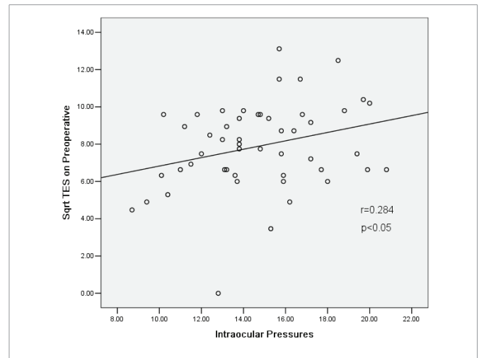
Figure 1: Correlation between Sqrt TES and intraocular pressures preoperative. There was positive correlation between Sqrt TES and intraocular pressures.
