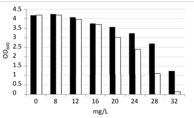
Figure 2: Dose-response curves of thioridazine racemic (TZR) and thioridazine (-) (-TZ (JEK47)). At OD 600 0.2 a culture of MSSA strain Newman was exposed to various concentrations of TZR or -TZ (0–32 mg/L). The OD 600 was measured after 3.7 hours of exposure is presented. Black bars; TZR, white bars; -TZ. The experiments were repeated twice and one set of data is presented. The raw data for figure 2 and data for additional time points (0.65, 1.1, 1.67, 2.7, 3.7, 4.65, 5.7 and 6.65 hours) can be found in the supporting information file S1_figure_2.pdf.
