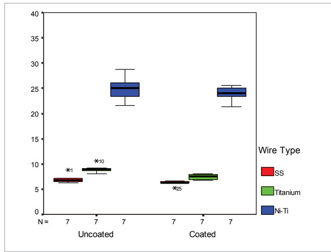
Graph 2: The Inter - group distribution of Elongation (Box - Plot).
