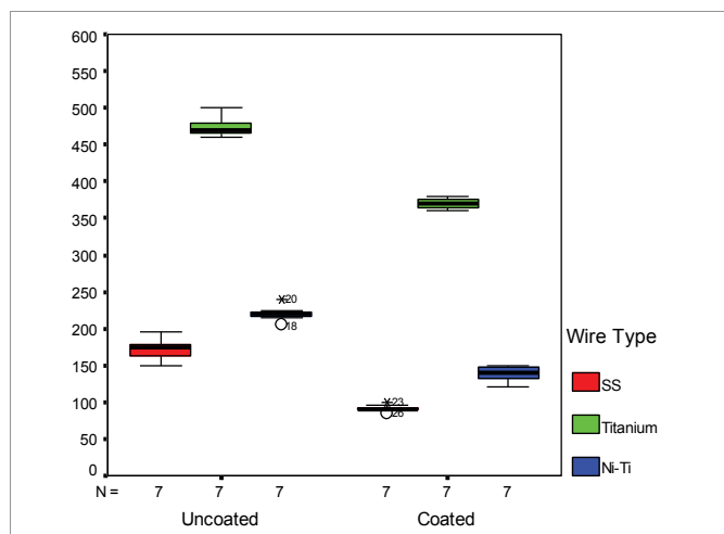
Graph 5: The Inter - group distribution of Frictional Resistance (Gms) (Box - Plot).
